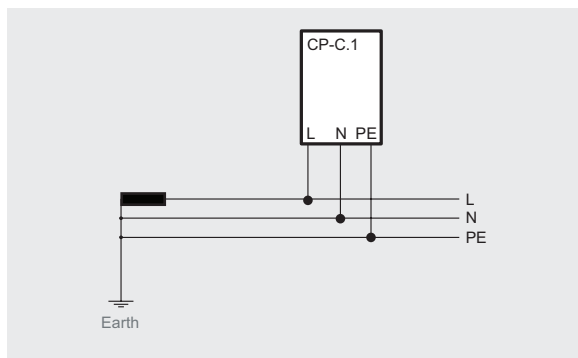
TN-S 1-phase
